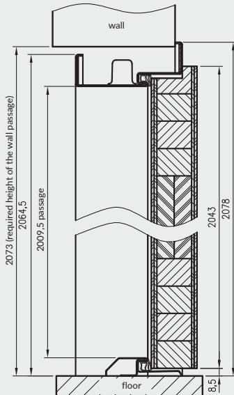
vertical cross-section of the Forca B door leaf
