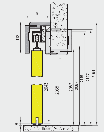
NT - vertical cross-section for tunnel with 80 mm architrave
