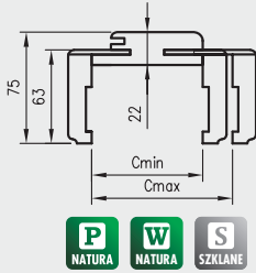
OR/ORC cross-section Natura with N63 architrave
