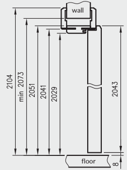
vertical cross-section of rebated door leaves
