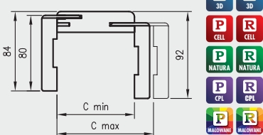
TUN cross-section with T63
