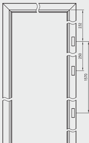
metal door frame - front view
