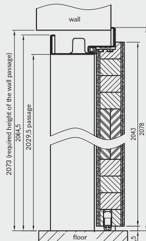
vertical cross-section ATHOS doors
