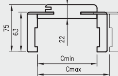
OR/ORC cross-section with T63 architrave
