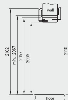
vertical cross-section of adjustable tunnel with T80
