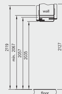
vertical cross-section of adjustable tunnel with T80
