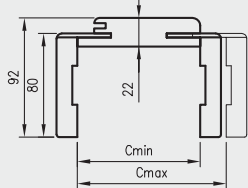
OR/ORC cross-section with T63 architrave
