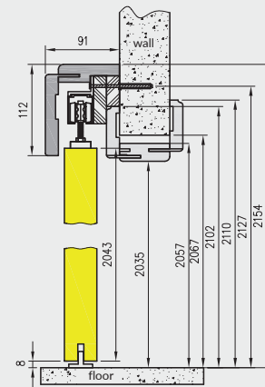
NT - vertical cross-section for tunnel with 63 mm architrave
