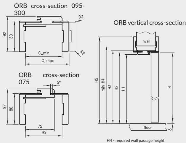
H4 - required wall passage height
