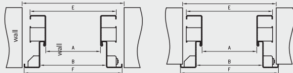
horizontal cross-section of door frame in the wall D (width of the opening in the wall)
