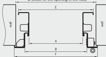
horizontal cross-section of door frame in the wall
