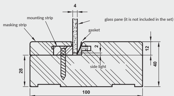
Fig. A cross-section of the transom light/sidelights
