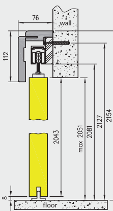
NS - vertical cross-section
