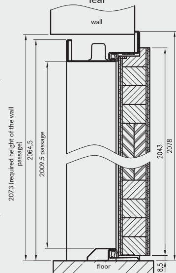
vertical cross-section FORCA door leaf
