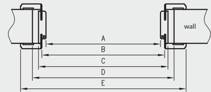
OR/ORC horizontal cross-section
