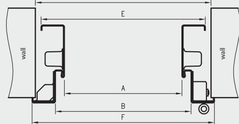
horizontal cross-section of door frame in the wall
