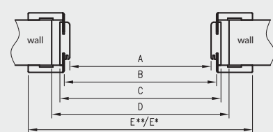
OR/ORC horizontal cross-section
