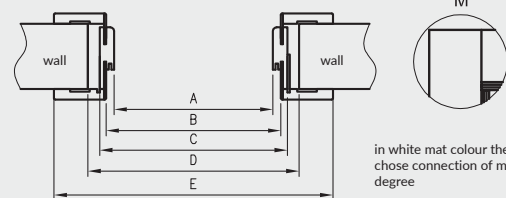
ORB horizontal cross-section
