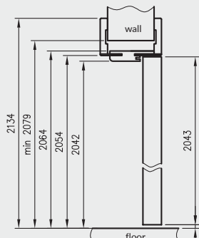
required wall passage height 2079mm
