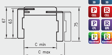
TUN cross-section with T63
