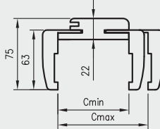
OR/ORC cross-section Natura with N63 architrave
