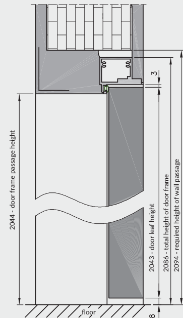
Sara Eco vertical cross-section
