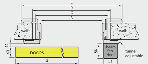
NT - horizontal cross-section (left system)
