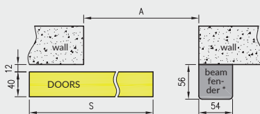
NS - horizontal cross-section (left system)
