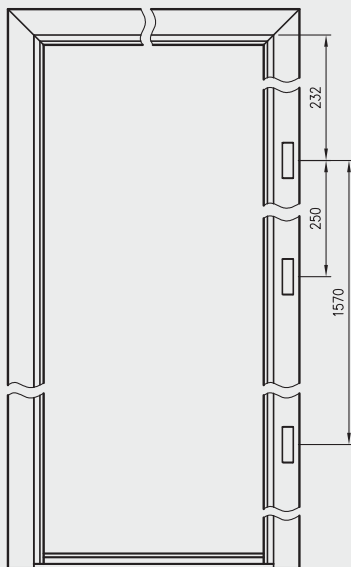
metal door frame - front view
