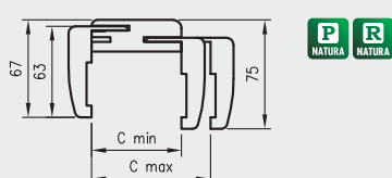
TUN cross-section with T80
