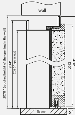
Vertical cross-section assembled by using mineral wool
