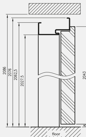
cross-section optional assembly method
