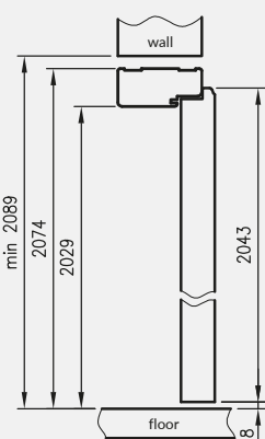
vertical cross-section of rebated door leaf
