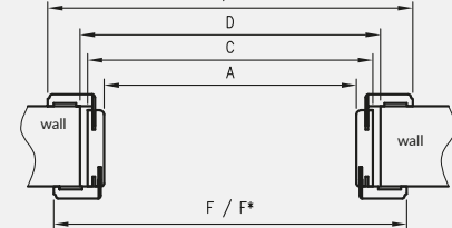
cross section of adjustable tunnel E / E*
