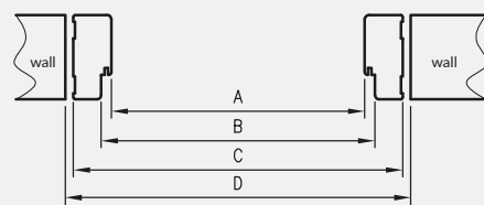
horizontal cross-section of fixed door frame
