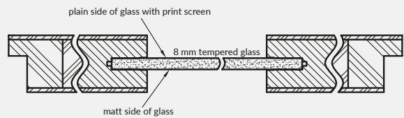
Horizontal cross-section of VETRO B5, B10-B11
