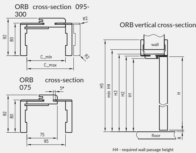
H4 - required wall passage height
