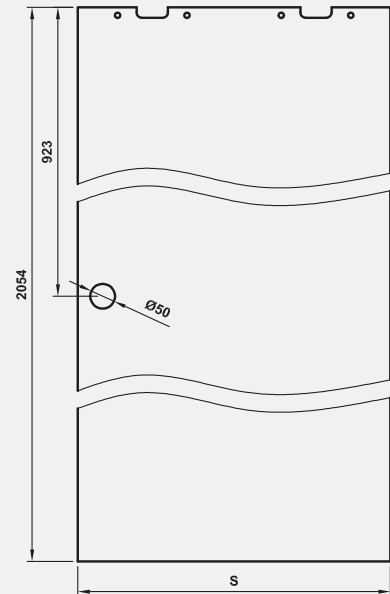
sliding glass door leaf
