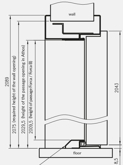
cross-section of an adjustable steel door frame
