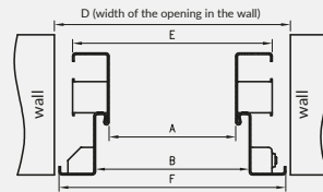
Dimensions for EI30 double leaf doors
