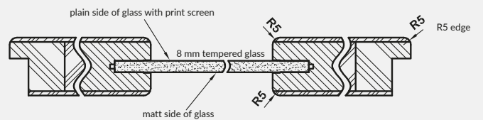
Horizontal cross-section of VETRO B5, B10-B11
