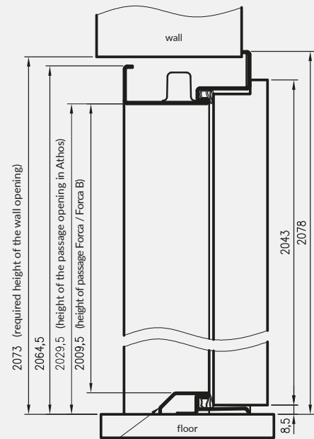
vertical cross-section
