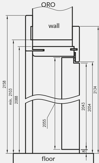
vertical cross-section of ORO
