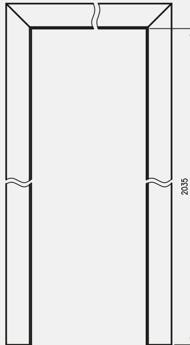
vertical cross-section of adjustable tunnel with T80
