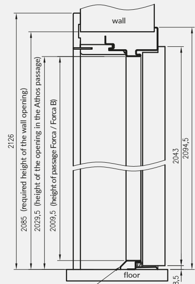
vertical cross-section
