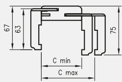
TUN Natura cross-section with N63
