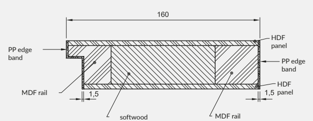
CROSS-SECTION OF VERTICAL STILE
