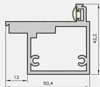
door frame profile with gasket
