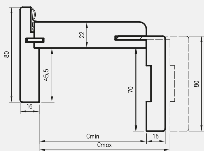
vertical cross-section of ORO
