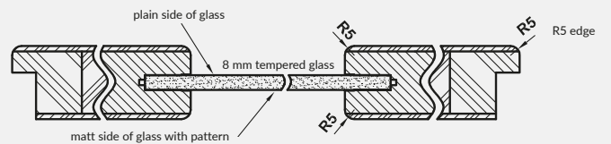
Horizontal cross-section of VETRO B5, B10-B11
