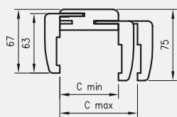
TUN cross-section with T80
