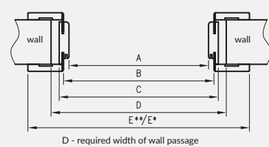
OR/ORC horizontal cross-section
