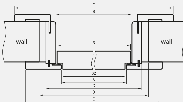
horizontal cross-section of ORO
