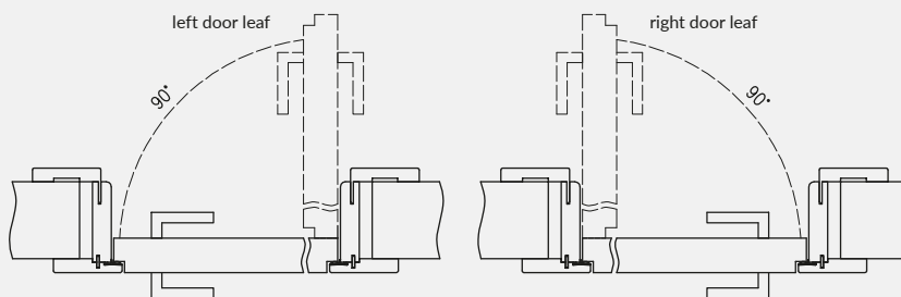
horizontal cross-section of ORO
