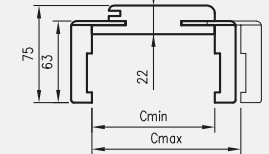
OR/ORC cross-section with T63 architrave
