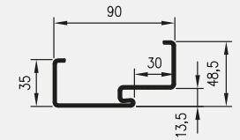
metal door frame cross-section
