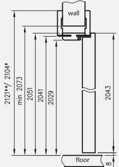
vertical cross-section of rebated door leaf with OR
