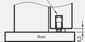
Fixed (steel) threshold for Forca and Forca B door leaves or dropping seal in Athos door leaves
