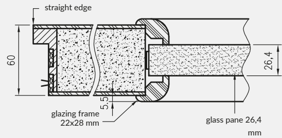
Fire resistant door leaf Olimp EI60
