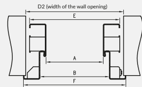
assembly cross-section by using concrete mortar
