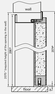
Vertical cross-section assembled by using concrete mortar
