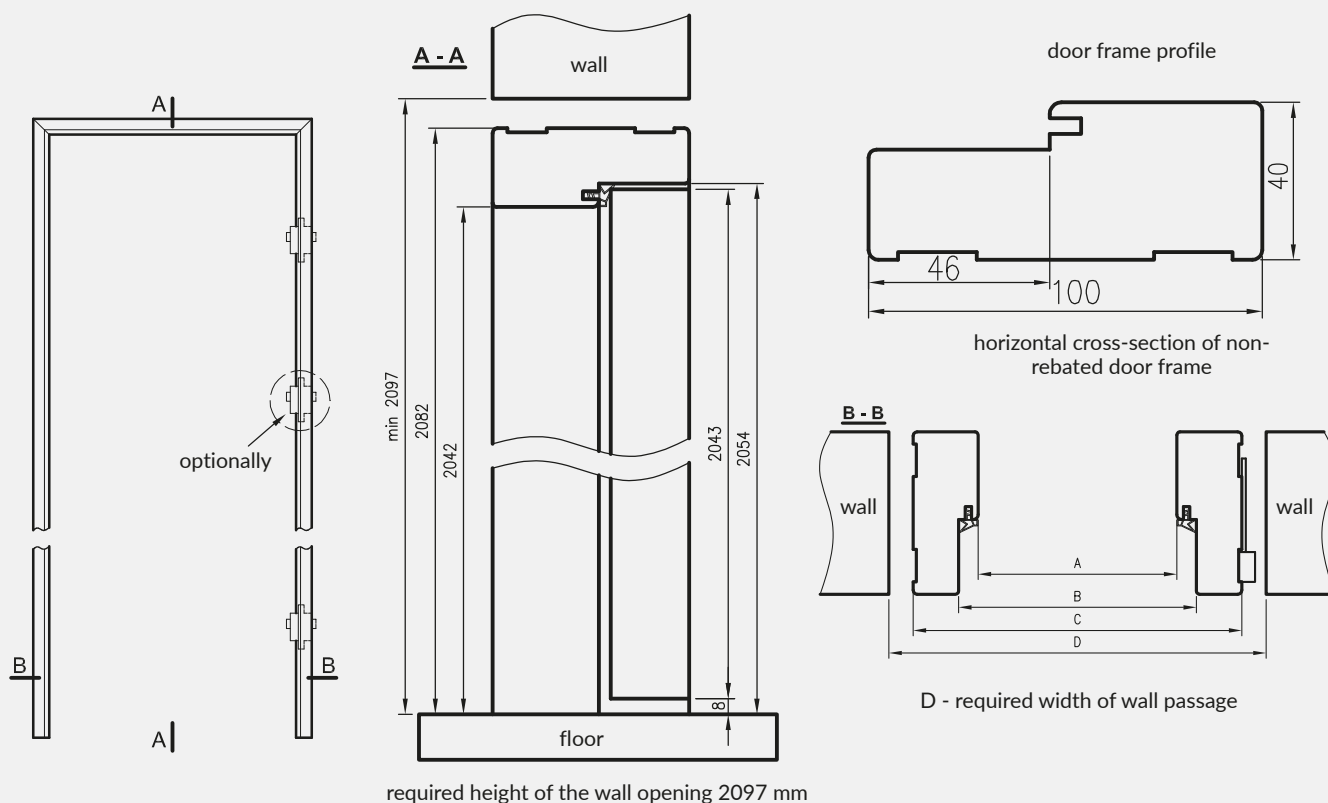
vertical cross-section OPB non-rebated door leaves
