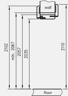
vertical cross-section of adjustable tunnel with T80
