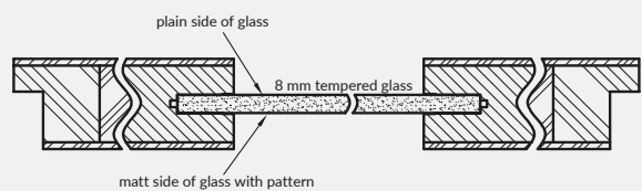
Horizontal cross-section of VETRO B5, B10-B11
