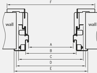
horizontal cross-section of door frame mounted in the wall
