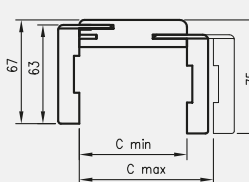
TUN cross-section with T63
