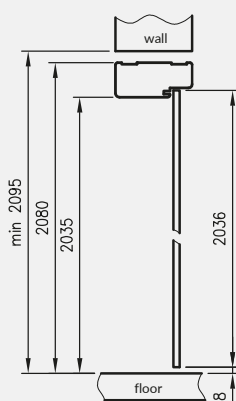
vertical cross-section glass doors
