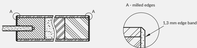
cross-section of stile in non-rebated door leaf
